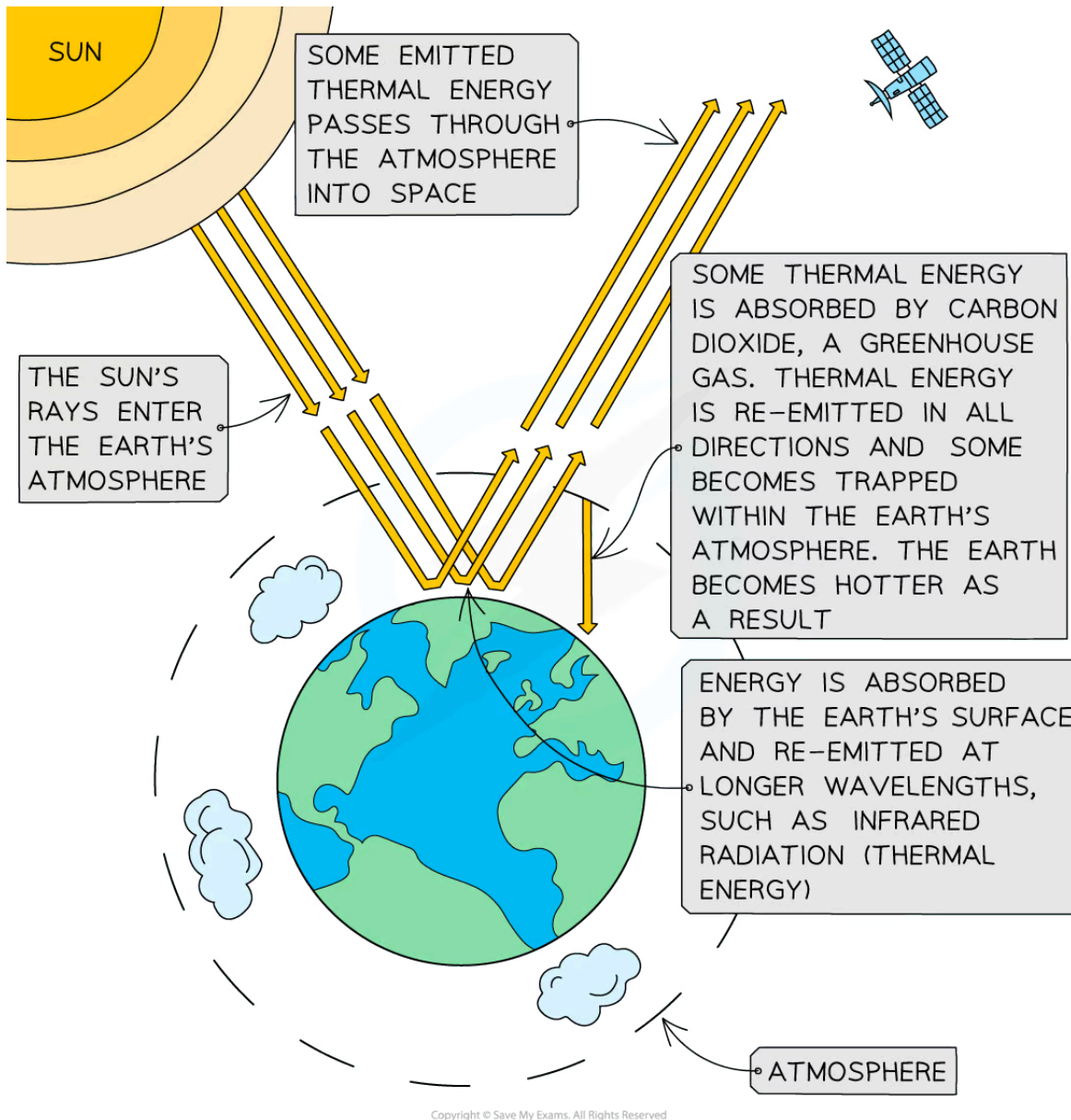
Diagram showing how the greenhouse effect occurs
