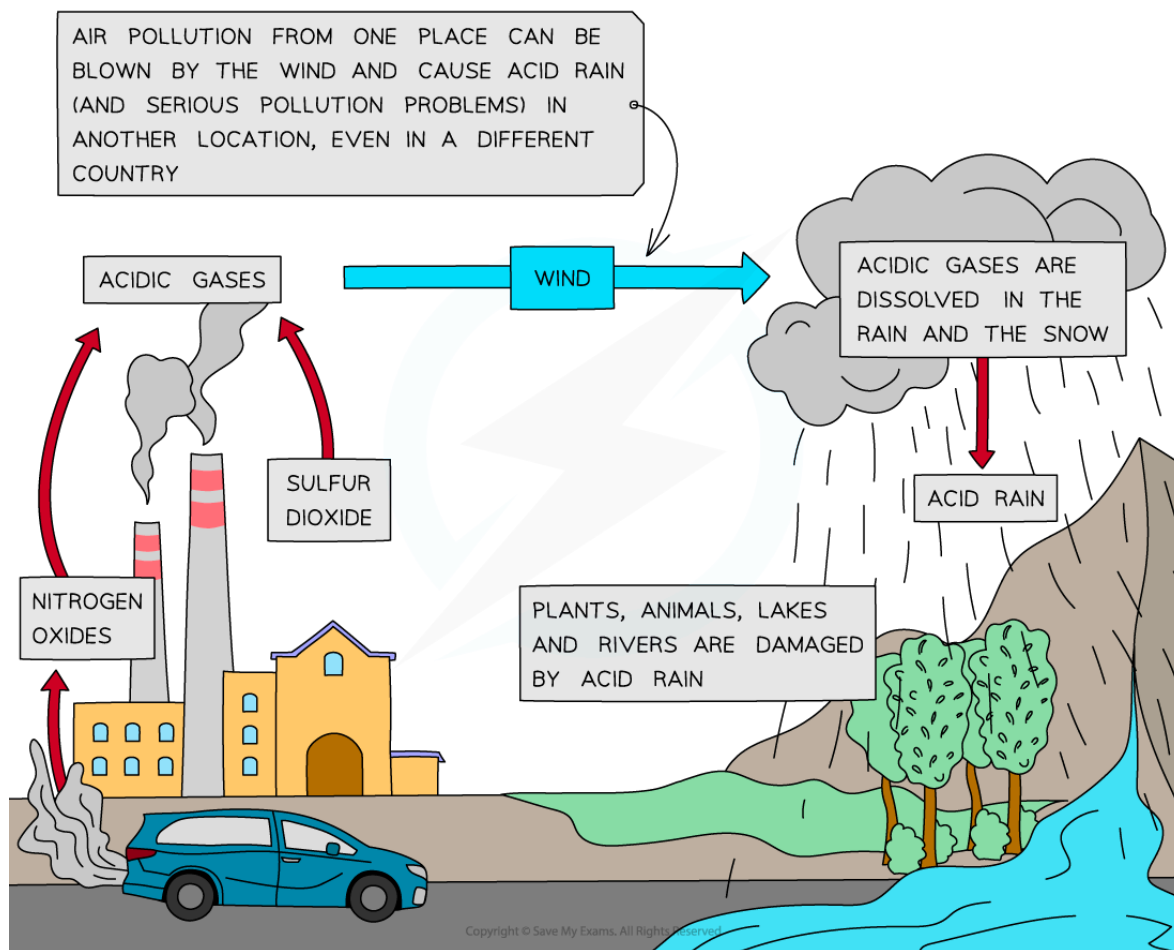
How acid rain is produced
